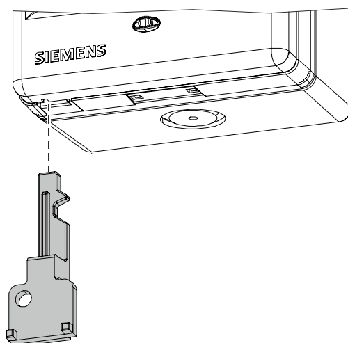
Using key FDMK295 to reset the manual call point (left) and open the housing (right)
