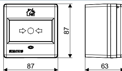
Radio manual call points FDM275 and FDM275(F)
