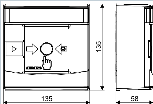
Radio manual call point FDM273
