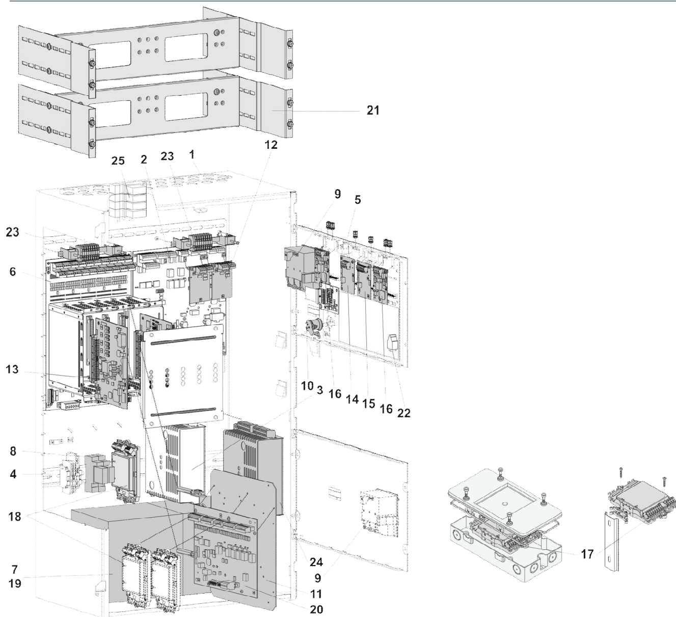
Layout of FC726
