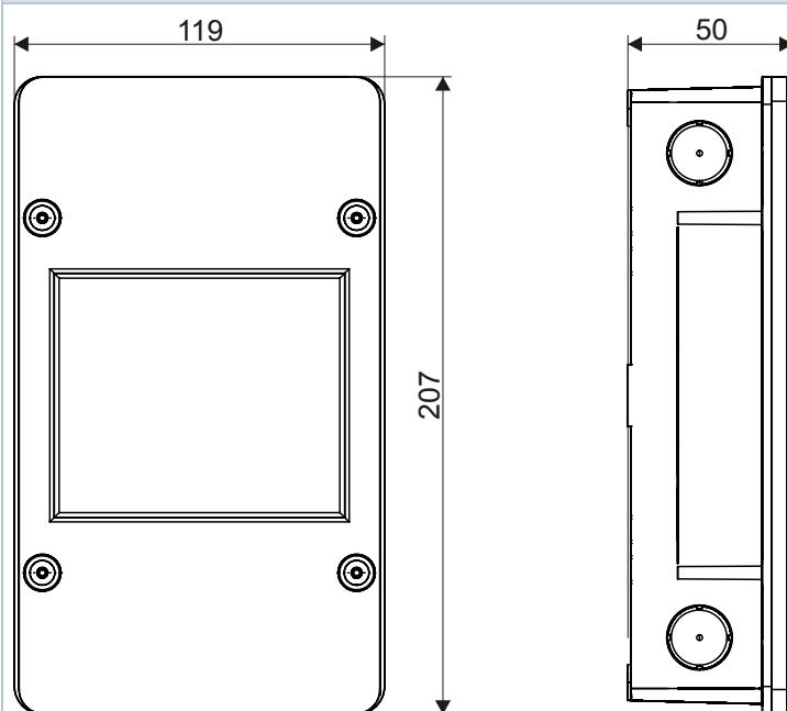
Housing FDCH221
